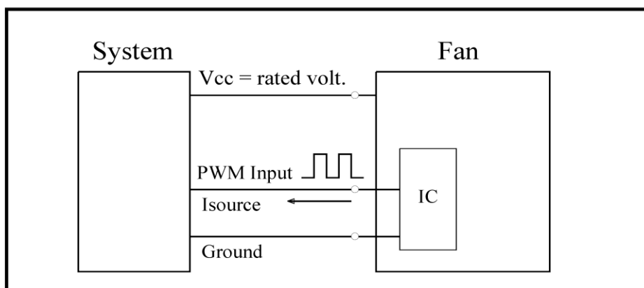
★PWM INPUT WAVEFORM
