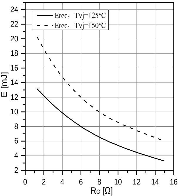
图10 二极管反向恢复损耗 Fig.10 Diode Reverse Recovery Energy Loss E_{rec} vs R_G , V_R=600\text{V} , I_F=450\text{A}
