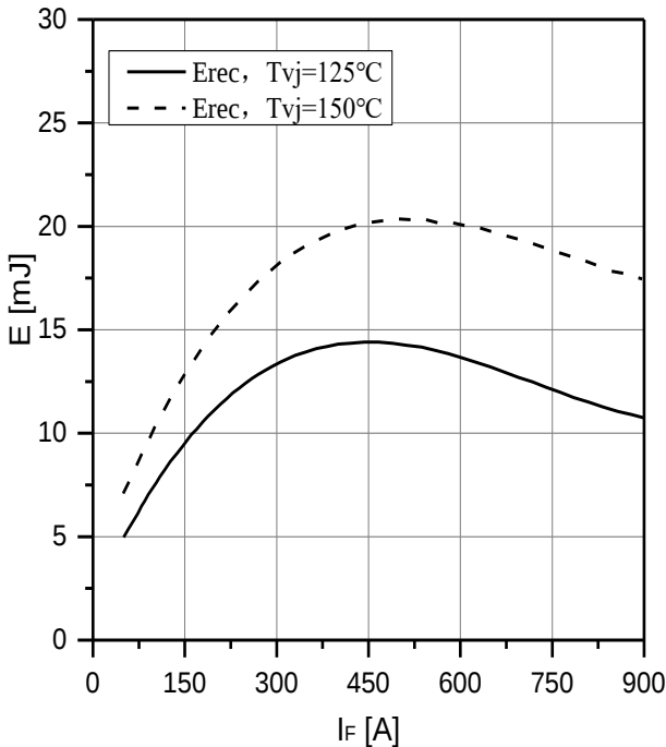
图9 二极管反向恢复损耗 Fig.9 Diode Reverse Recovery Energy Loss E_{rec} vs I_F , V_R=600\text{V} , R_G=1.3\Omega
